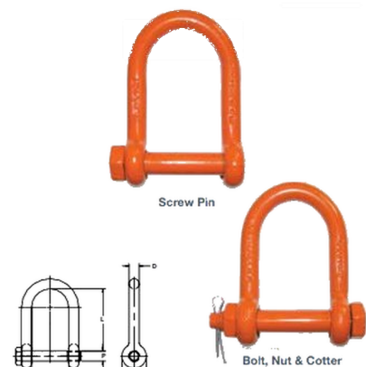
SCREW PIN (TOP) · BOLT, NUT & COTTER (BOTTOM)
